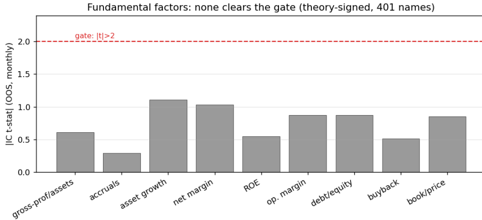
Figure 4: Fundamental factors through the gate (401 names, 2015–2024, monthly horizon, theory-signed). Every bar is below the |t| = 2 line: no fundamental factor clears the gate. The verdict is unchanged at quarterly, semiannual, and annual horizons.
