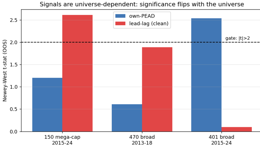
Figure 3: The central fragility result. Newey–West t -statistic of own-PEAD and the clean lead–lag across three universes. Significance flips with the universe: own-PEAD clears the gate only on the broad mid-cap-inclusive universe, the lead–lag only on the narrow mega-cap one. Neither is robust.
