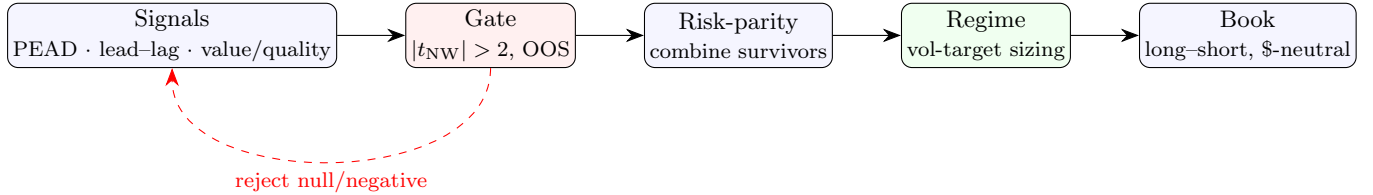
Figure 1: The pipeline. Candidate signals (point-in-time, from free EDGAR data) must pass an economic-P&L gate before a risk-parity combiner; a regime layer sizes the surviving book. The gate is what protects performance: a signal that fails it is discarded, not down-weighted.
