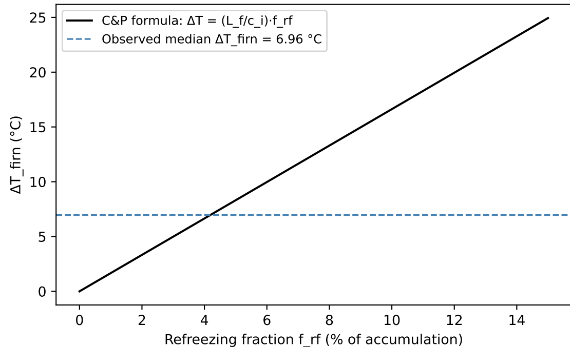
Cuffey & Paterson formula vs observed median
