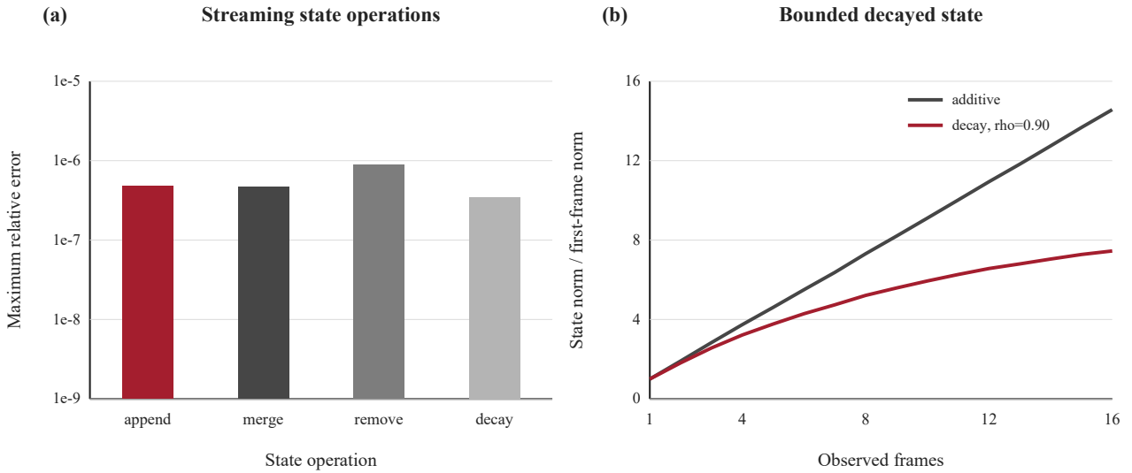
Fig. 3. Streaming state operations. (a) Maximum relative errors for append/merge, frame removal, and exponential decay, measured against independently reconstructed FWP states on 32 ShapeNetPart objects. (b) Ordinary addition increases the state magnitude with the number of frames, while exponential decay limits the influence of older frames without changing state size.
