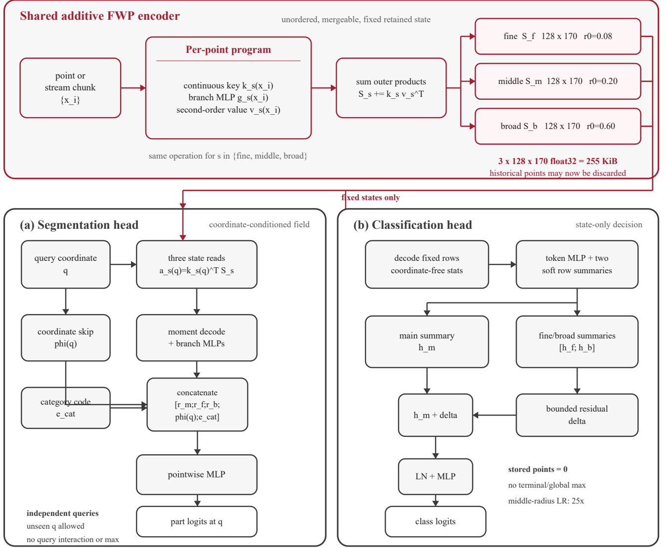
Fig. 1. PointProgrammerNet architecture. The shared encoder writes each observation into three equal-size additive FWP states, after which the historical point list can be discarded. For segmentation, the states are read at a query coordinate and combined with a direct coordinate skip. For classification, soft row summaries from the fine and broad states form a bounded residual around the middle-state summary. Neither head pools over decoded points.
