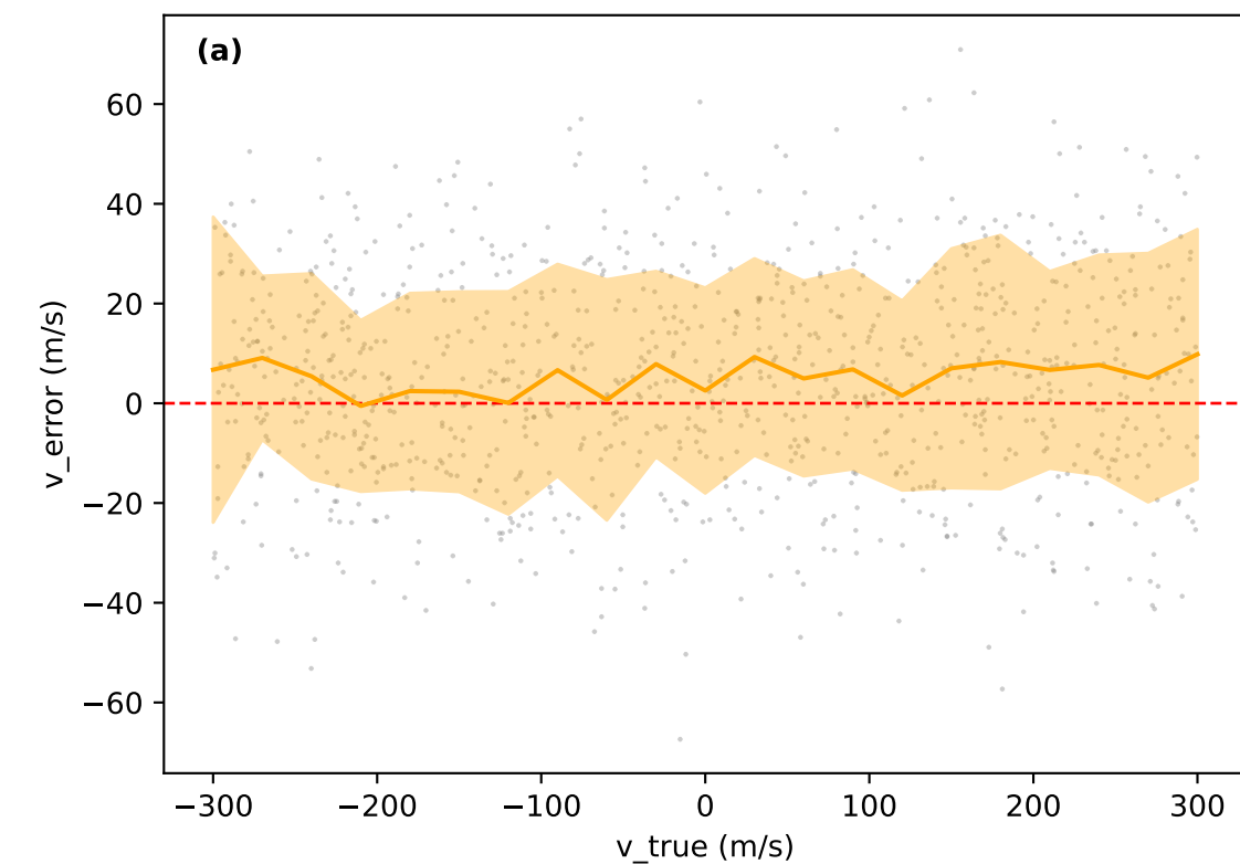
Simulation 2: Biases Over Wind Speed and Temperature (SNR = 5, N = 1,000)
