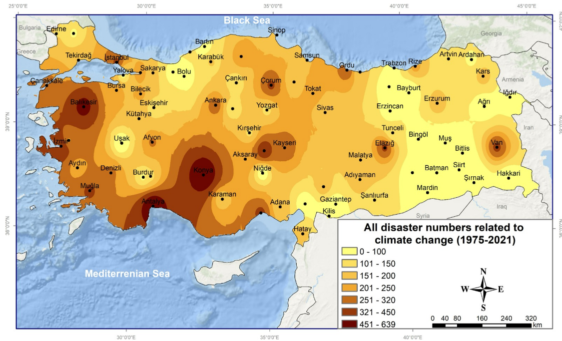
Figure 1: Total Climate Events in Türkiye from 1975 to 2021
