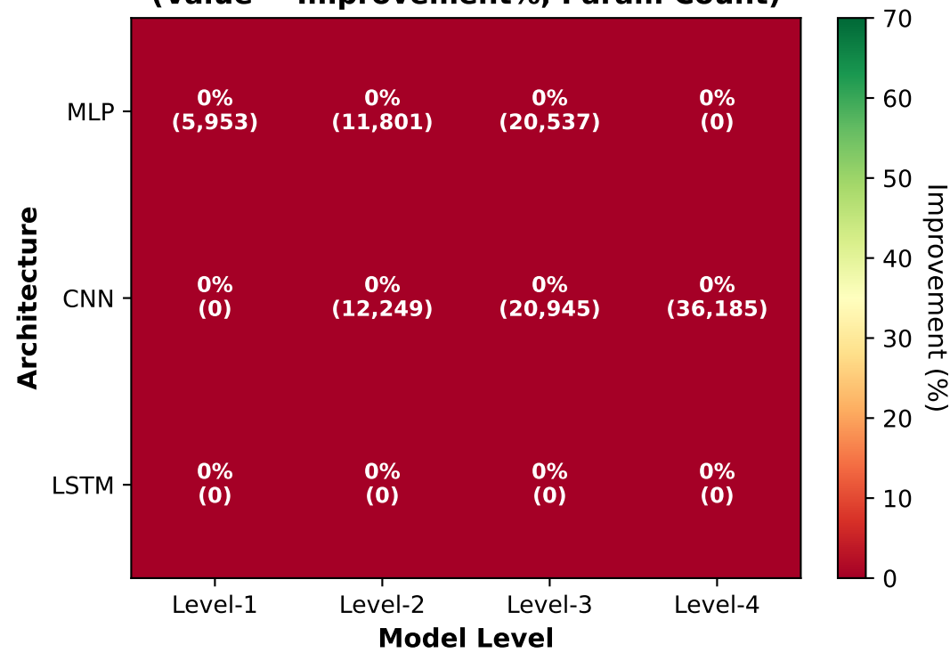
(b) Improvement × Architecture × Level (Value = Improvement%, Param Count)
