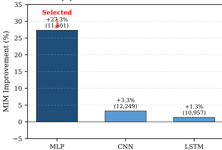
(A) L1: Architecture Selection
