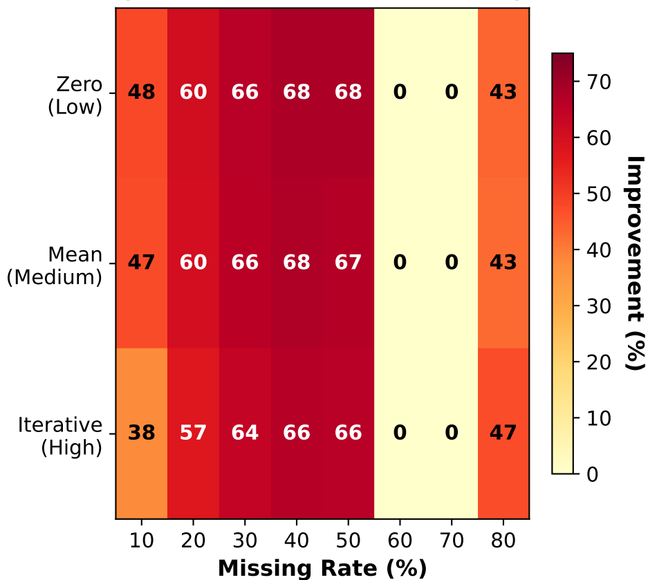
(c) Quality × Missing Rate Interaction (Warmer = Better MIM Effect)
