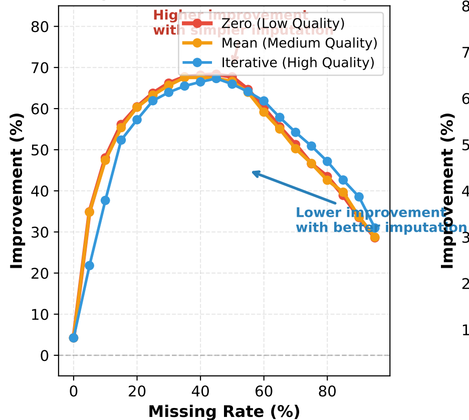
(a) MIM Effectiveness Gradient (Zero > Mean > Iterative)
