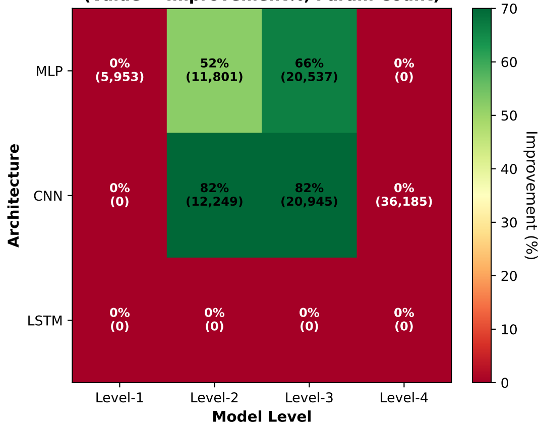
(b) Improvement \times Architecture \times Level (Value = Improvement%, Param Count)
