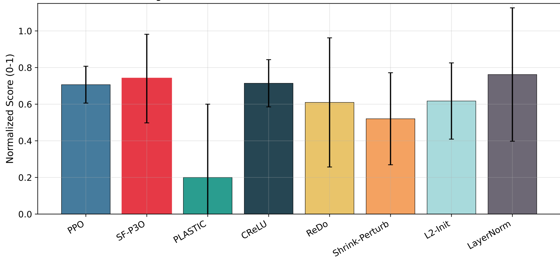
Figure 6: Normalized Performance across All Environments
