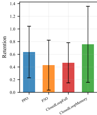
Hopper→Walker2d→Hopper: Phase 3 Summary
