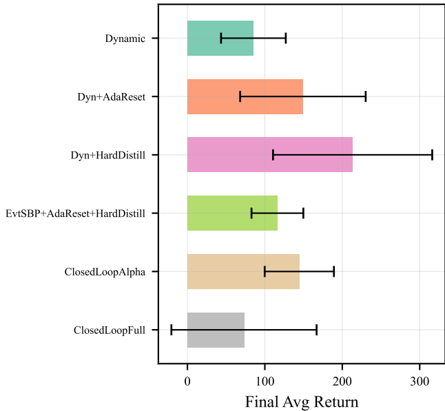
Walker2d
