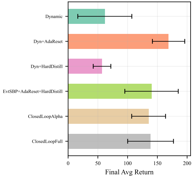
Hopper
