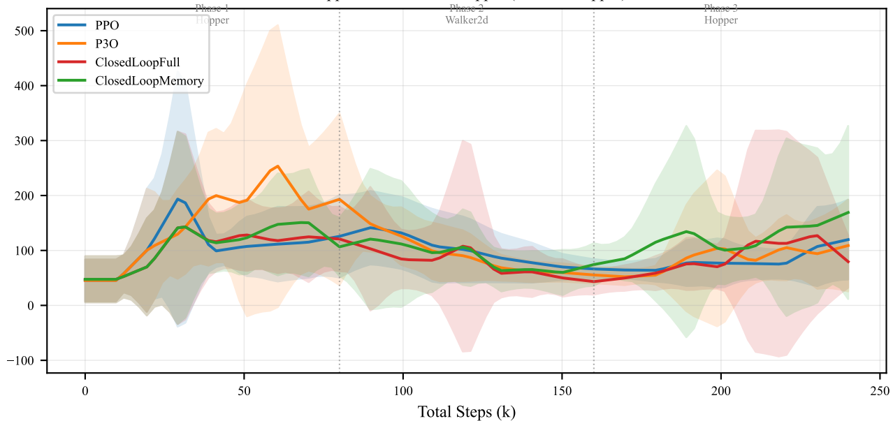
Hopper→Walker2d→Hopper (Eval on Hopper)
