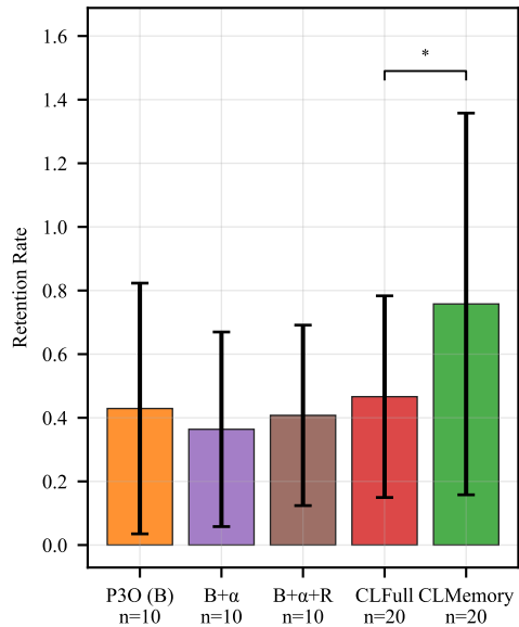
Retention Rate
