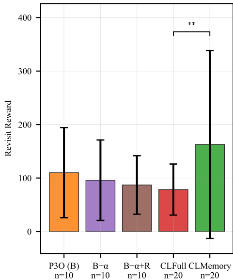
Revisit Reward
