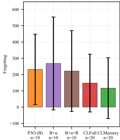
Forgetting
