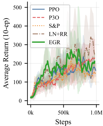
Hopper
