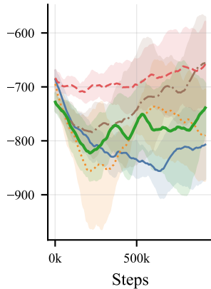
HalfCheetah
