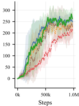
Walker2d
