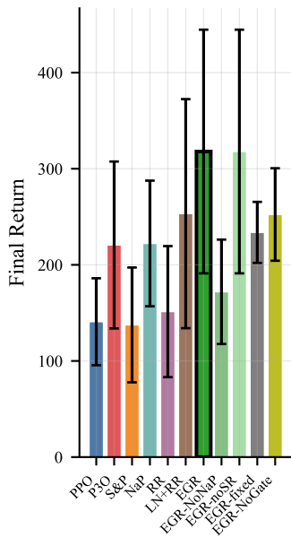
Hopper
