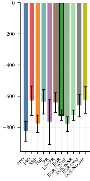
HalfCheetah
