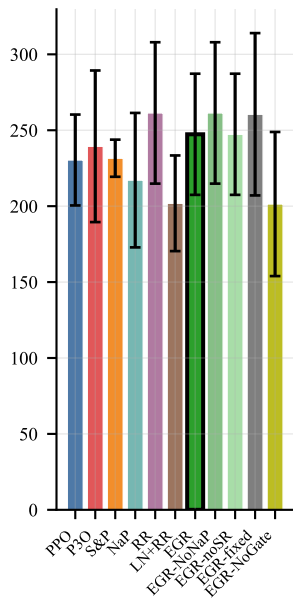
Walker2d
