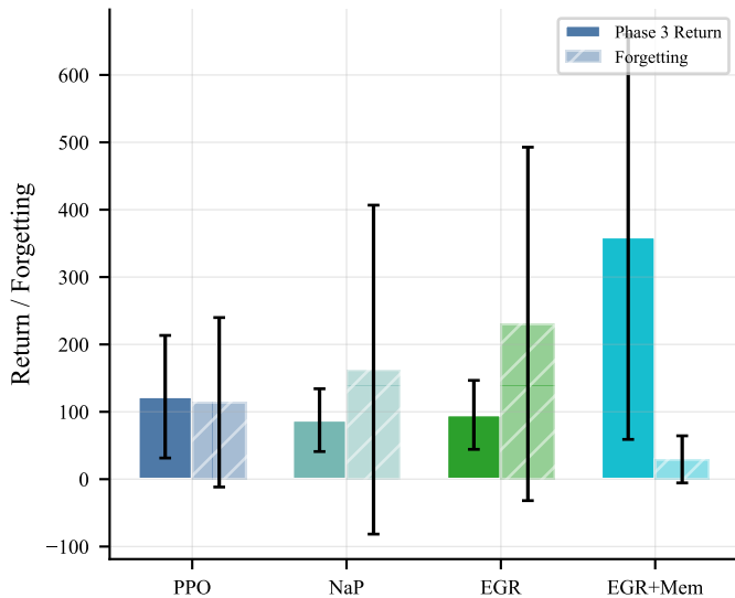
Hopper→Walker2d→Hopper
