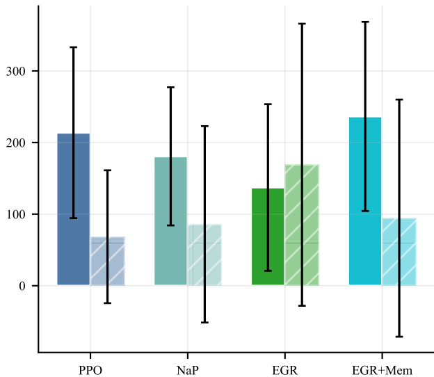
Walker2d→HalfCheetah→Walker2d
