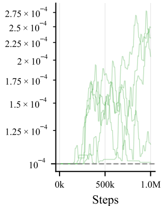
HalfCheetah
