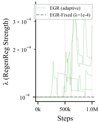
Hopper
