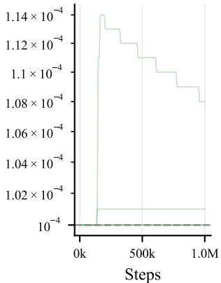
Walker2d
