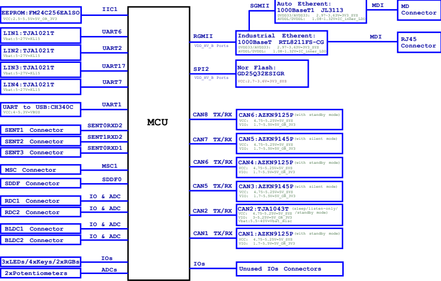
1, System Block Diagram
