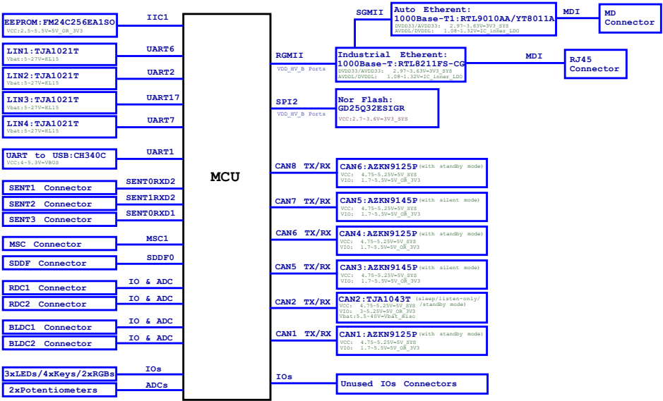
1, System Block Diagram
