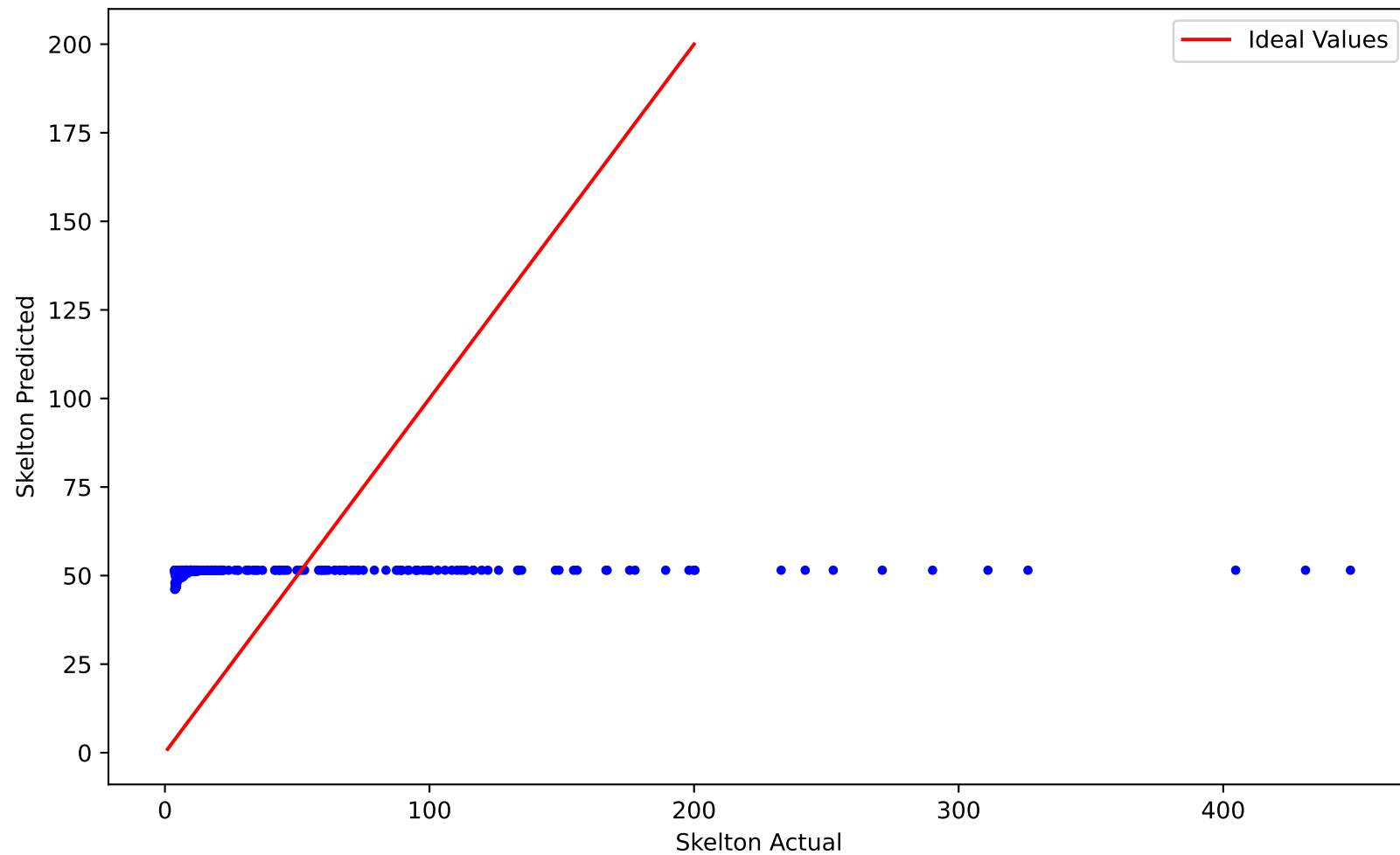
Correlation Plot
