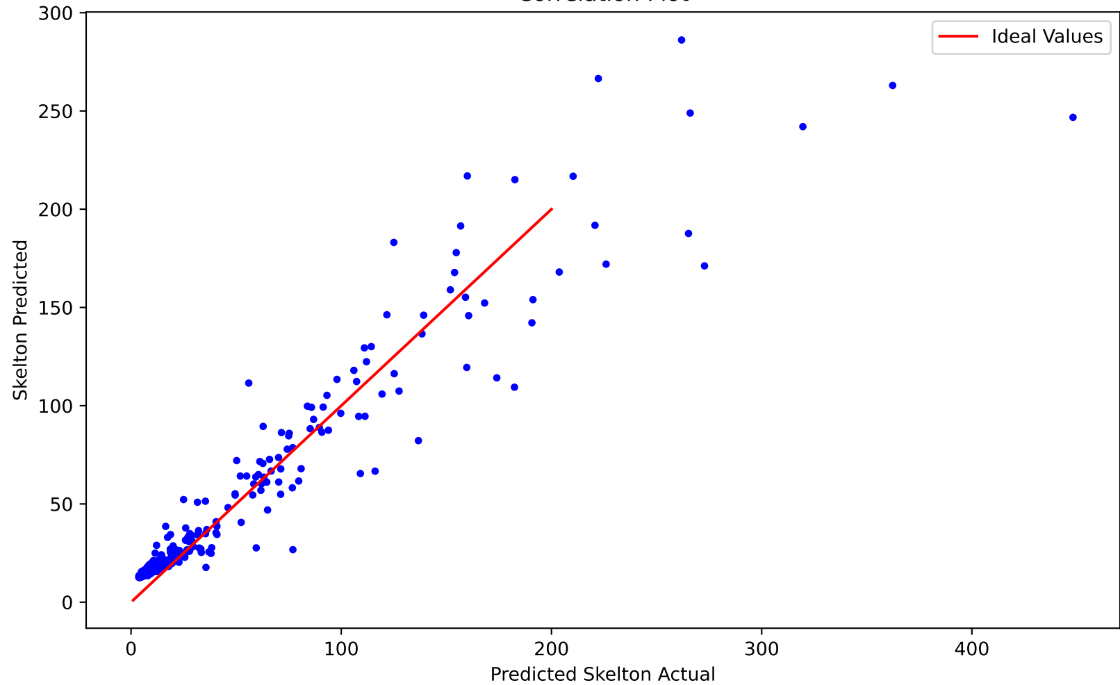
Correlation Plot
