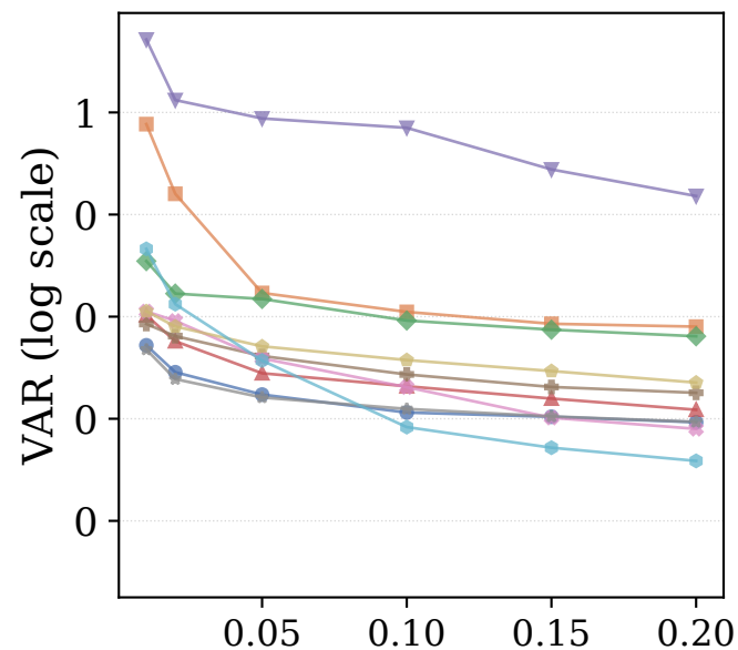
MR
