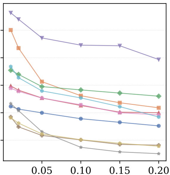
RF
