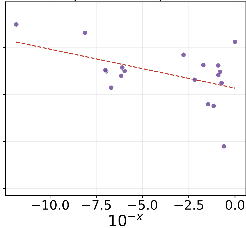
t_c = 2 ( \rho = -0.37 , p = 0.124 )
