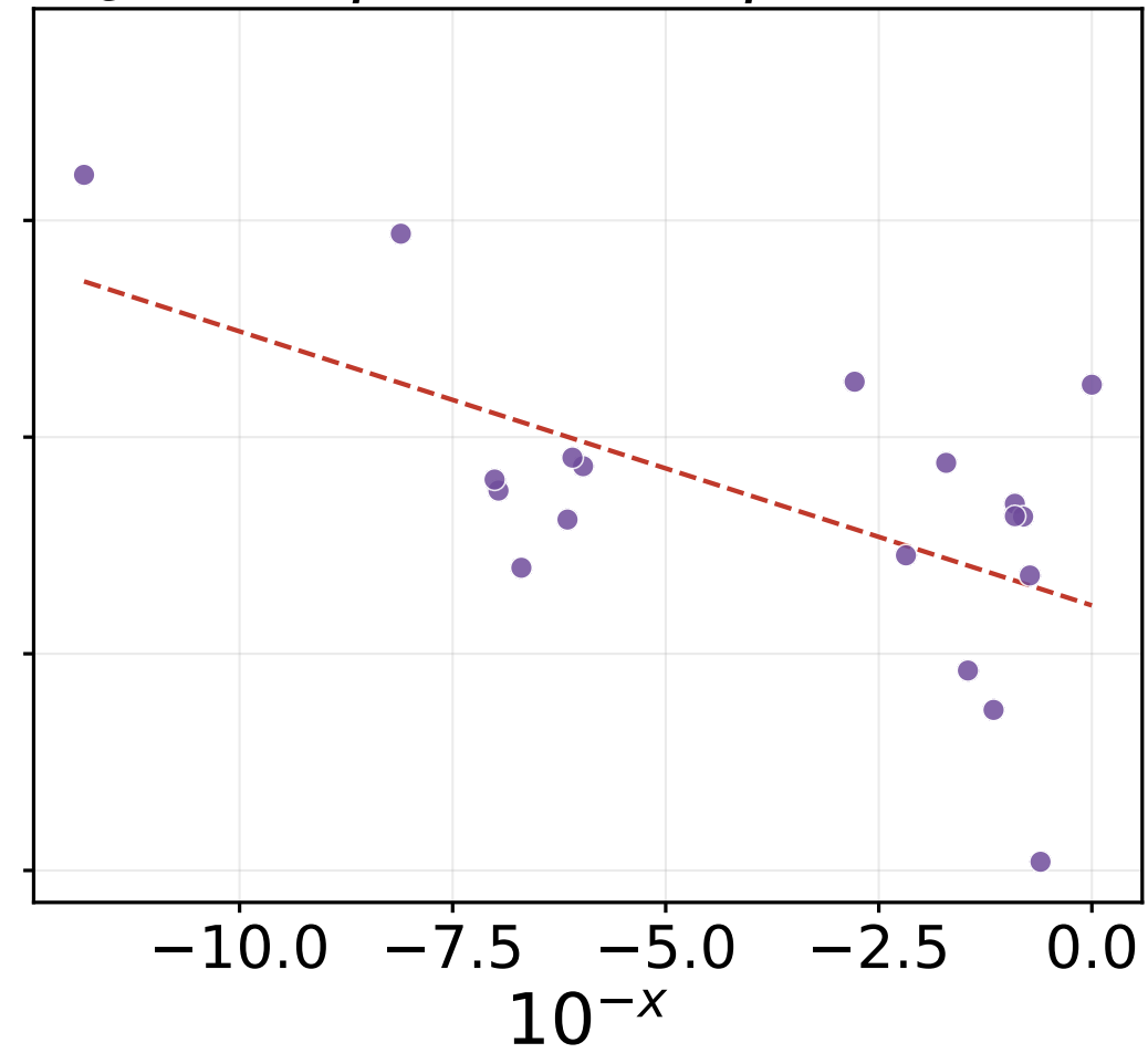
t_c = 3 ( \rho = -0.47 , p = 0.043 )
