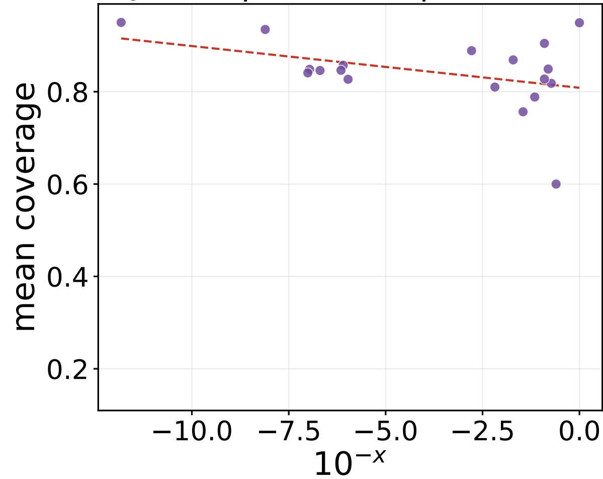
t_c = 1 ( \rho = -0.30 , p = 0.208 )
