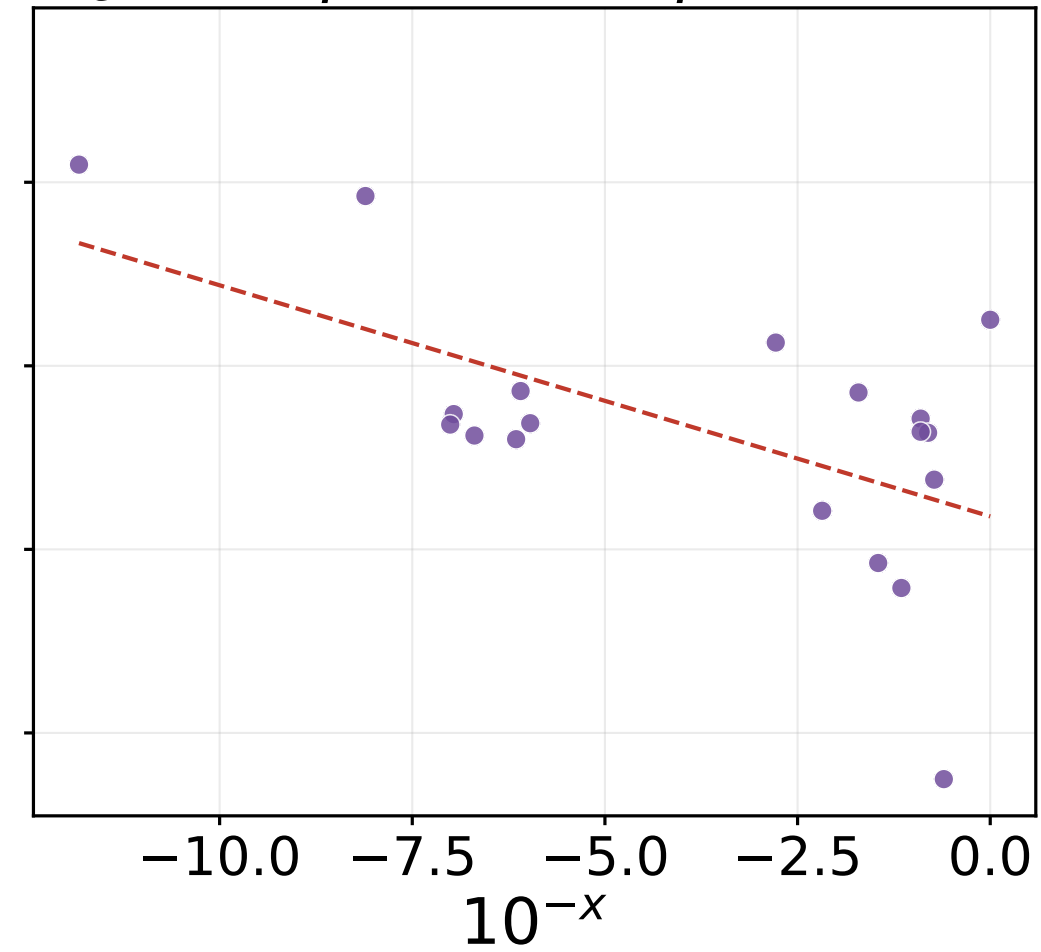
t_c = 3 ( \rho = -0.42 , p = 0.072 )
