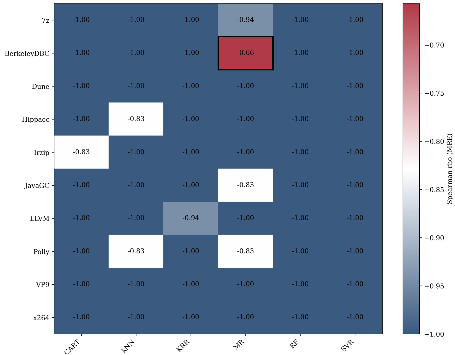
Spearman rho (MRE vs. proportion)
