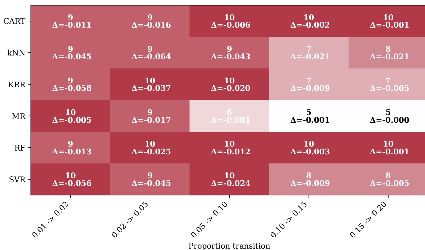
Number of systems with BH-significant MRE reduction per step
