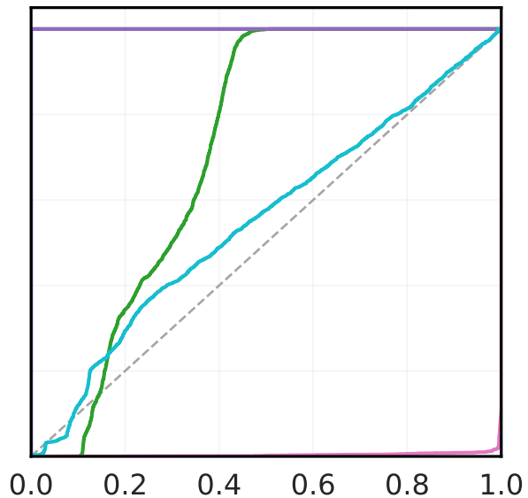
Couette
