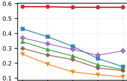
Graph-SST2
