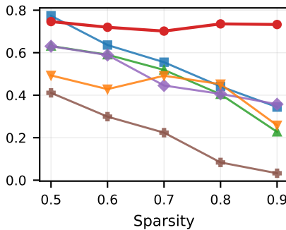
BA-House-OR-Grid
