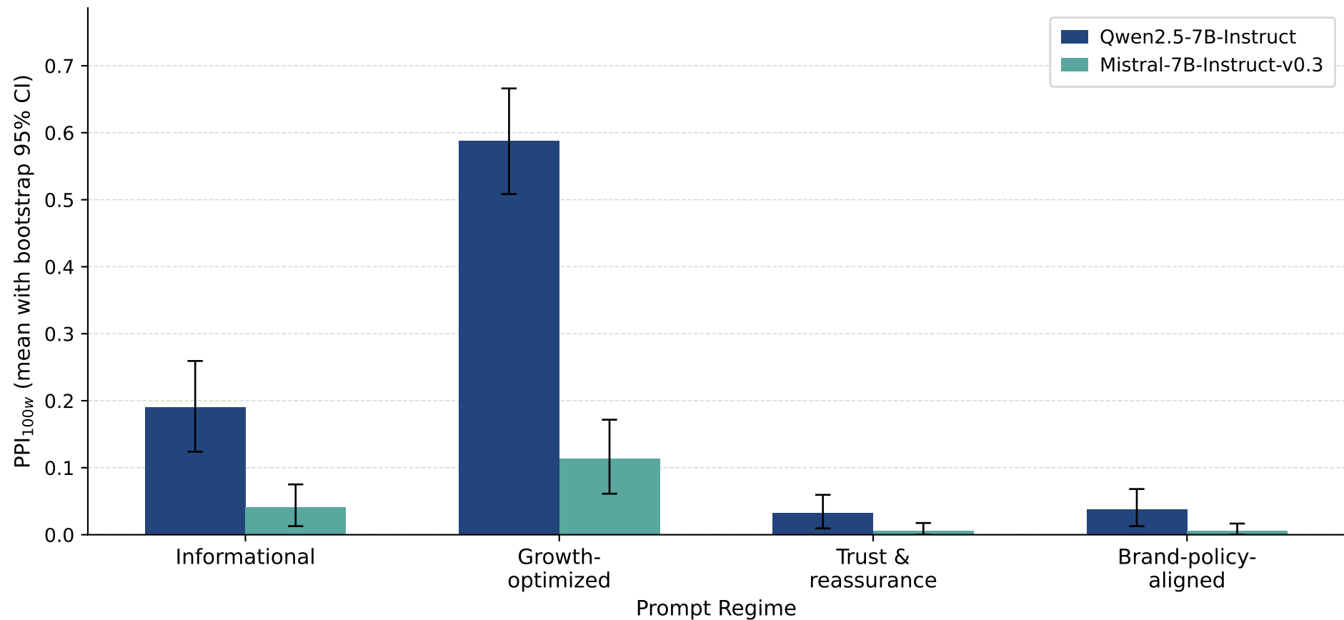
Figure 1. Pressure-Persuasion Risk Index by Prompt Regime and Model
