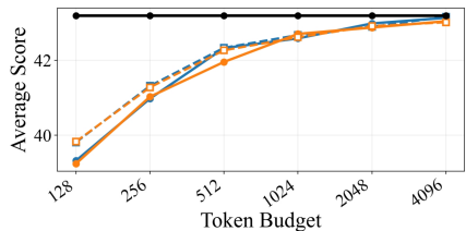
(a) LongBench, Mistral-7b-instruct-v0.2
