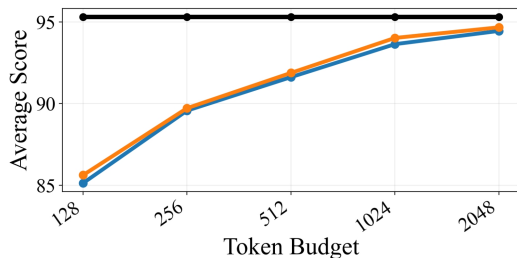
(h) RULER-8K, Llama3.1-8b-instruct
