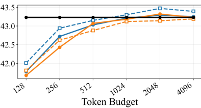
(b) LongBench, Llama3-8b-instruct
