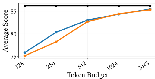
(f) RULER-16K, Mistral-7b-instruct-v0.2
