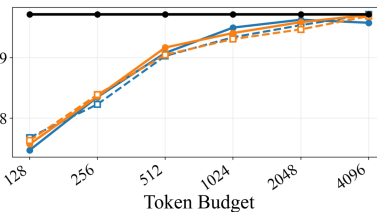
(c) LongBench, Llama3.1-8b-instruct
