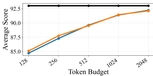
(i) RULER-16K, Llama3.1-8b-instruct
