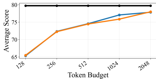
(g) RULER-32K, Mistral-7b-instruct-v0.2
