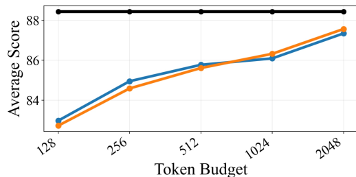
(j) RULER-32K, Llama3.1-8b-instruct
