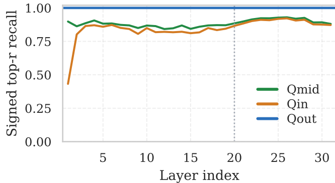
Query fidelity by layer
