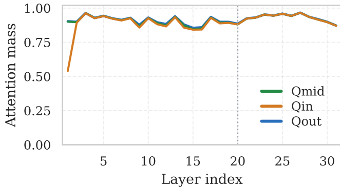
Routing fidelity by layer
