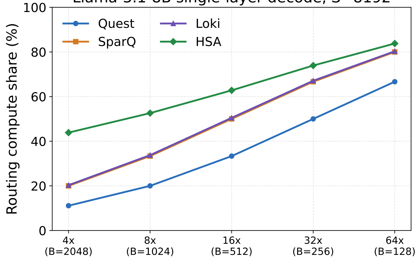
Llama-3.1-8B single-layer decode, S=8192
