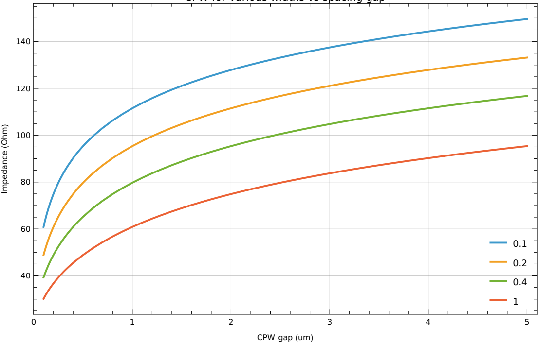
CPW for various widths vs spacing gap
