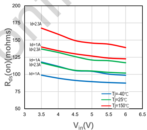
Figure 2-10 Static drain-source on resistance vs input voltage (part 1)
