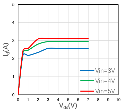
Figure 2-23 Output characteristics
