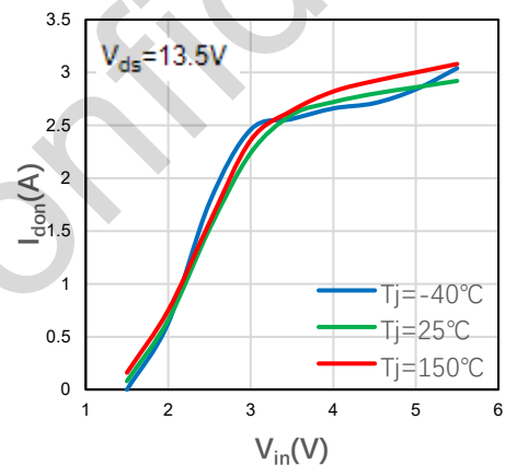
Figure 2-14 Transfer characteristics
