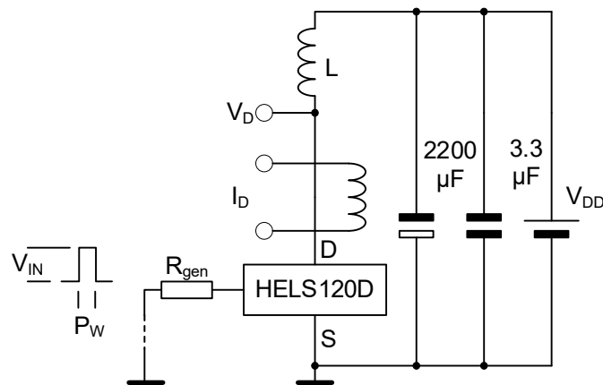
Figure 2-4 Unclamped inductive load test circuits
