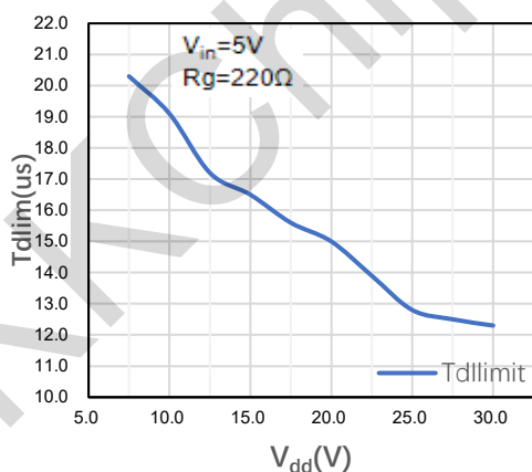
Figure 2-27 Step response current limit
