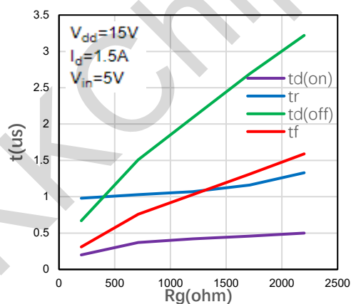
Figure 2-21 Switching time resistive load (part 1)
