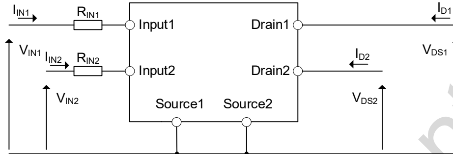
Figure 2-1 Current and voltage conventions
