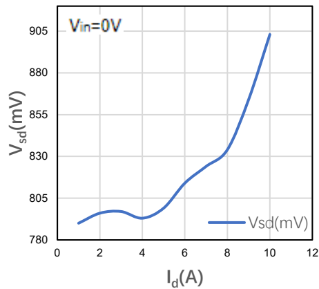
Figure 2-7 Source-drain diode forward characteristics
