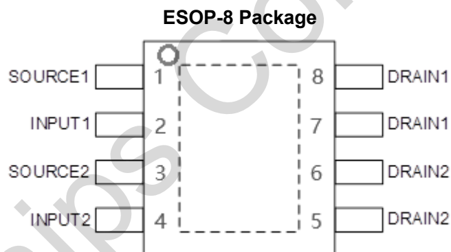
Figure 1-2 Configuration diagram (top view)
