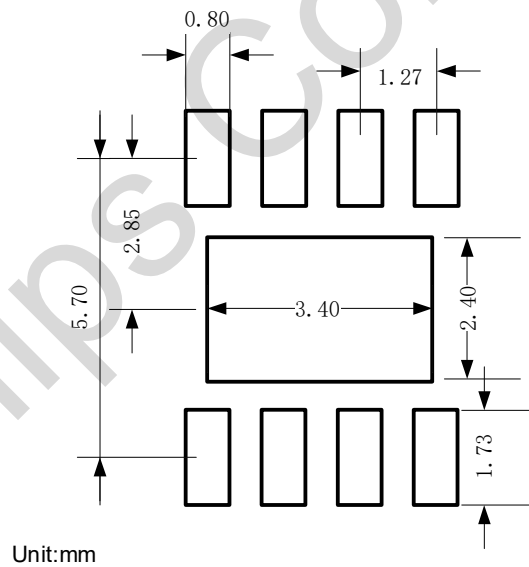
Figure 6-1 Recommended pad size
