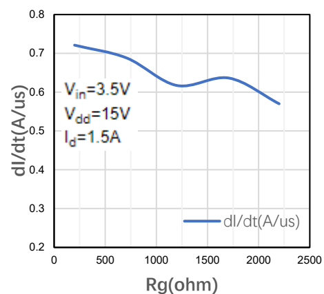
Figure 2-16 Turn-on current slope (part 2)
