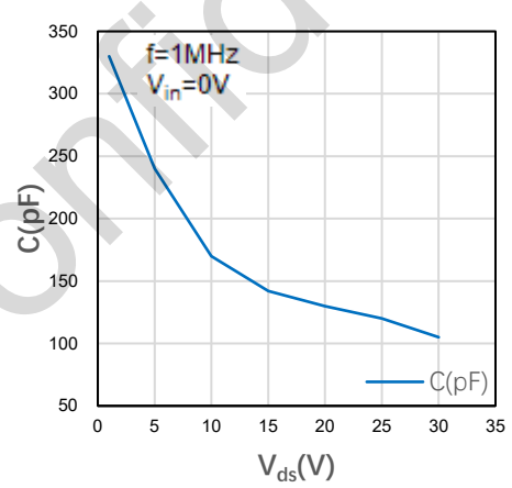
Figure 2-20 Capacitance variations
