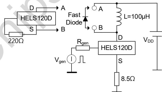
Figure 2-3 Test circuit for diode recovery times
