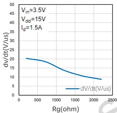
Figure 2-19 Turn-off drain-source voltage slope (part 2)
