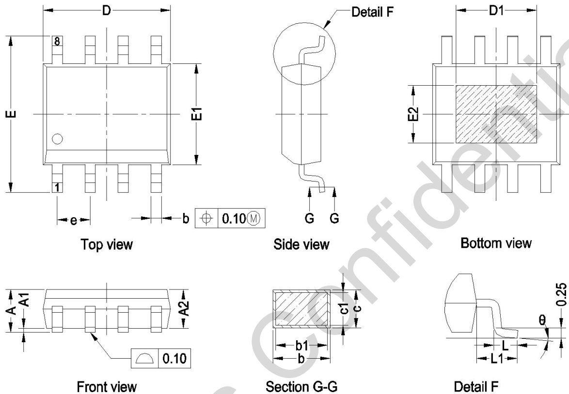
Figure 4-1 ESOP-8 package dimension
