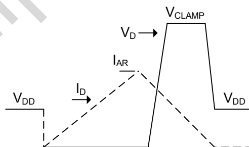
Figure 2-6 Unclamped inductive waveforms
