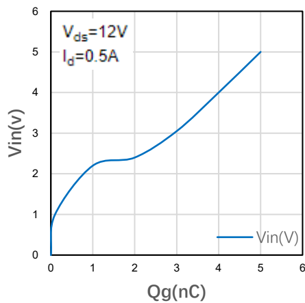
Figure 2-17 Input voltage vs input charge
