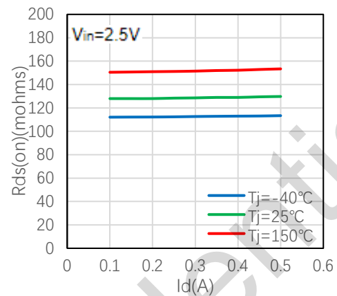
Figure 2-8 Static drain-source on resistance
