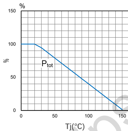
Figure 2-9 Derating curve
