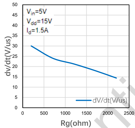
Figure 2-18 Turn-off drain-source voltage slope (part 1)
