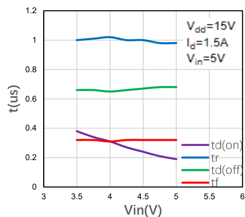
Figure 2-22 Switching time resistive load (part 2)
