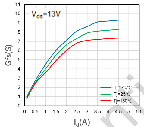
Figure 2-12 Transconductance
