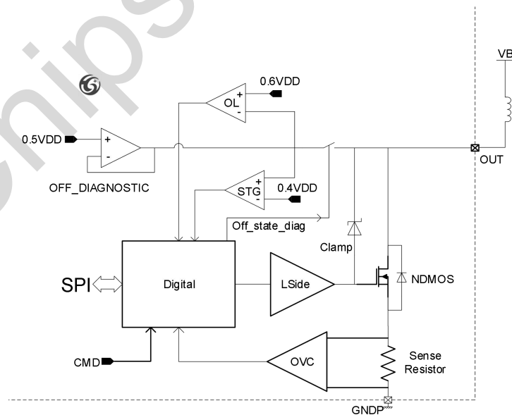
Figure 3-7 Low-side driver block diagram
