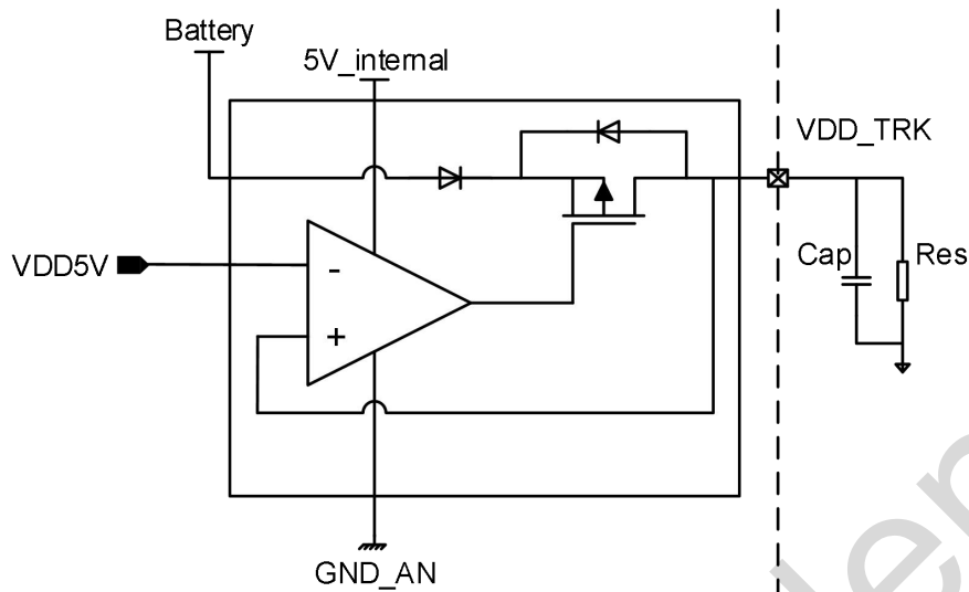
Figure 3-5 tracking regulator block diagram
