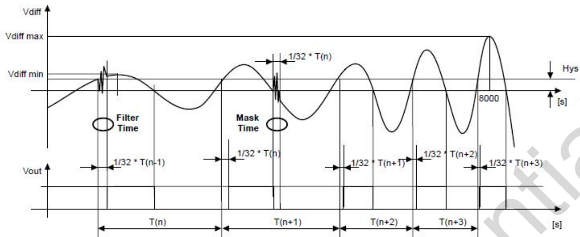
Figure 4-15 Auto-adaptive time filter behavior 2
