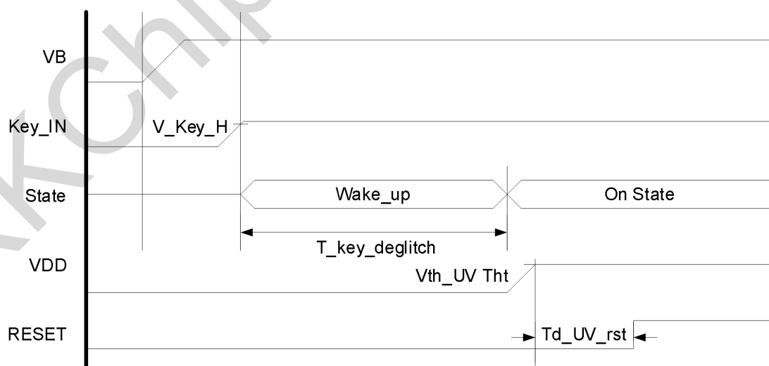
Figure 4-1 Power-up sequence
