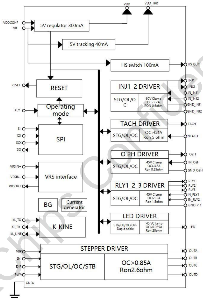
Figure 1-1 Block diagram
