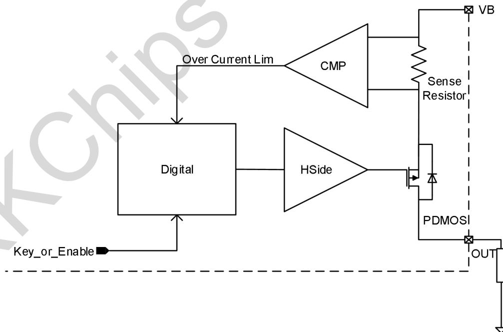
Figure 3-6 High-side driver block diagram
