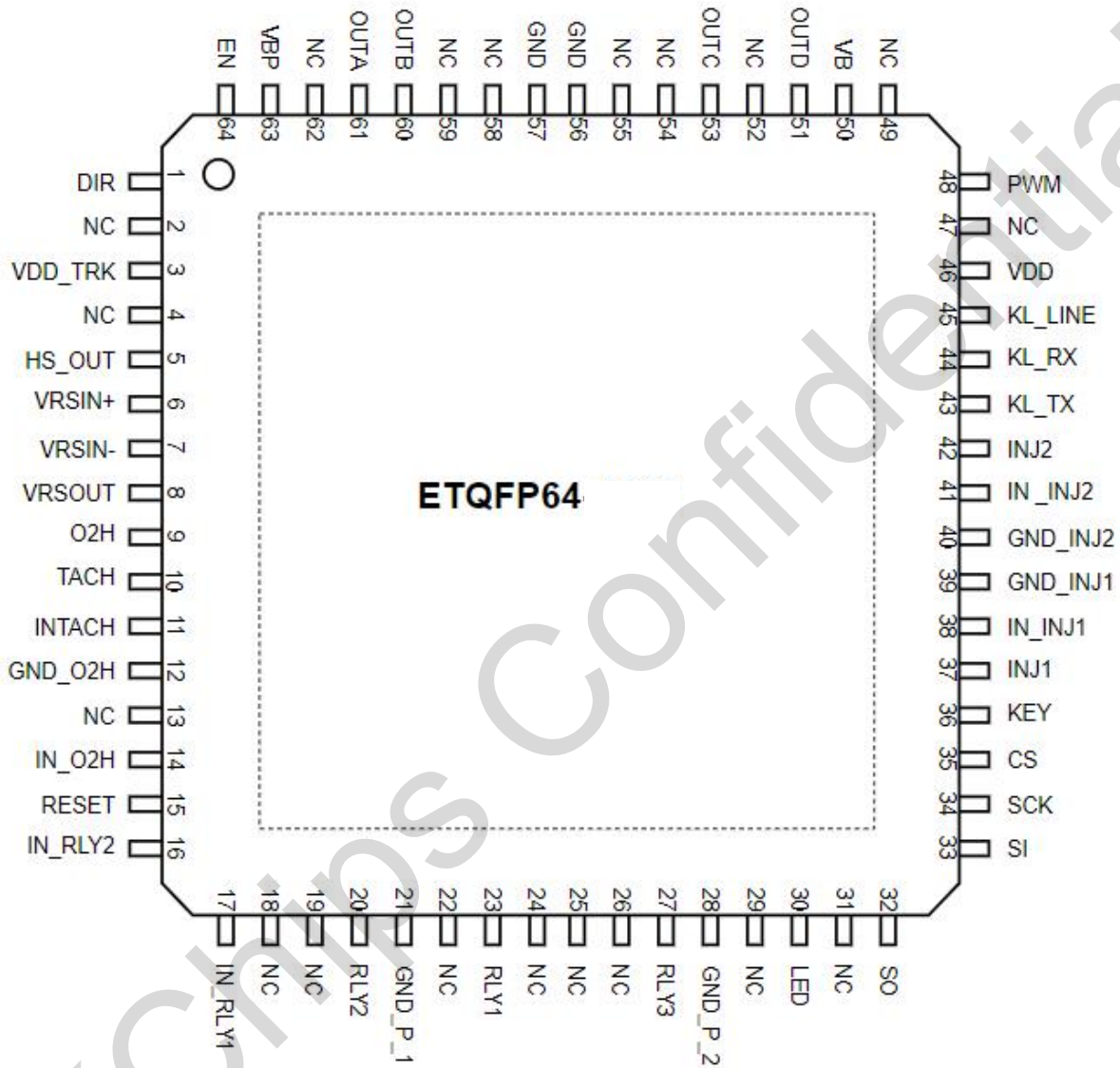
Figure 1-2 PIN OUT(64pin ETQFP64)
