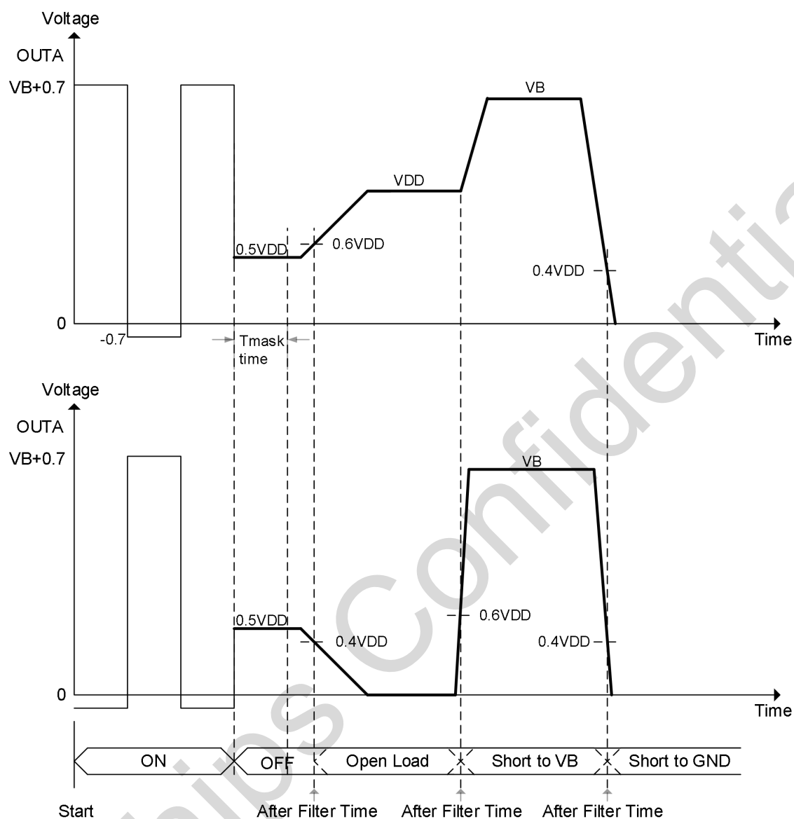
Figure 4-6 Stepper motor driver diagnosis time diagram
