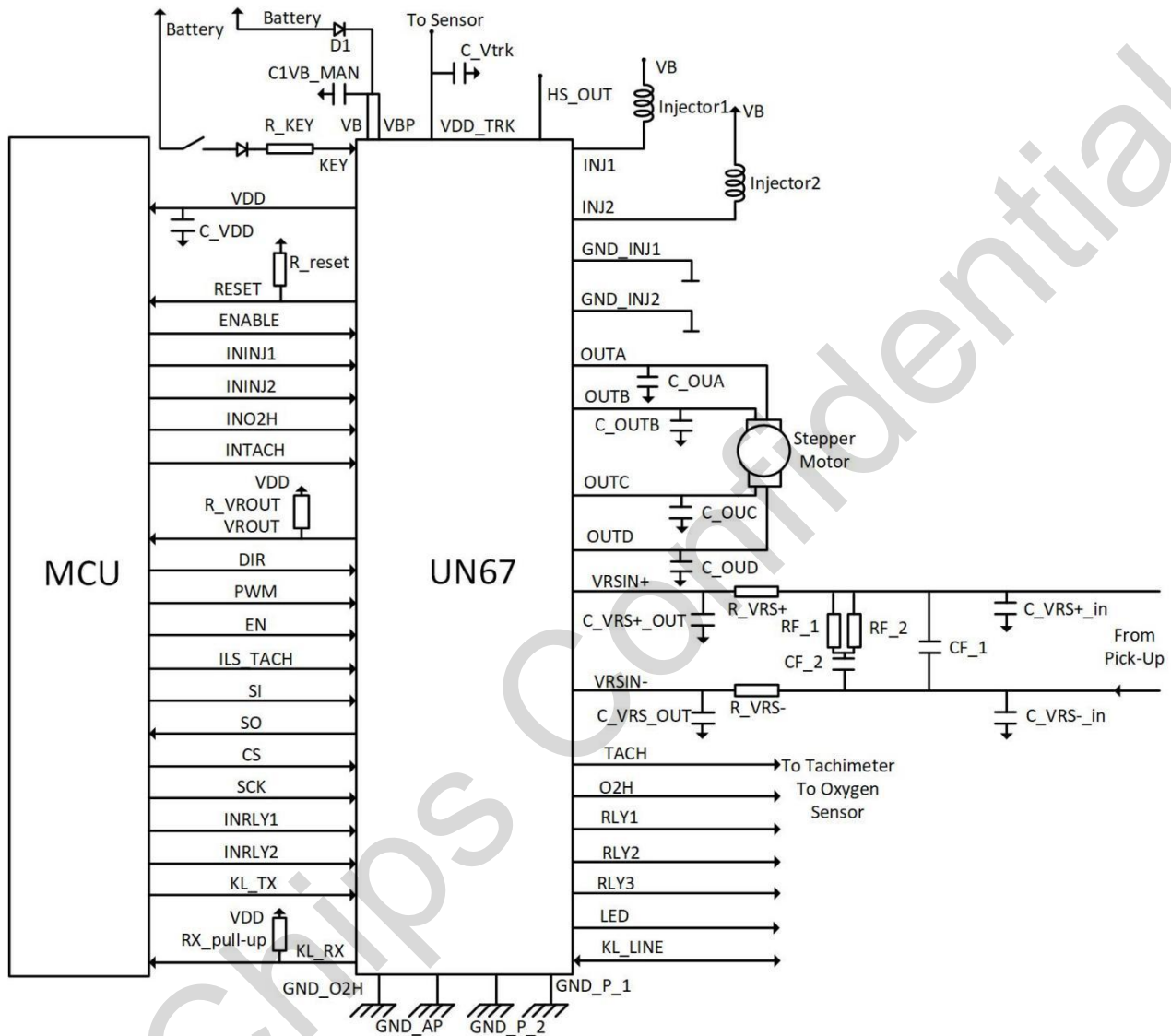
Figure 5-1 Application circuit
