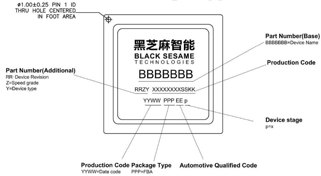
Figure 1-2 Marking Diagram
