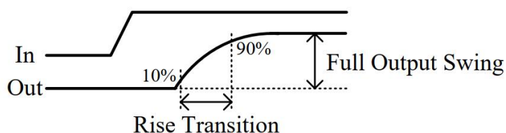
Figure 4-4 Output transition time waveform
