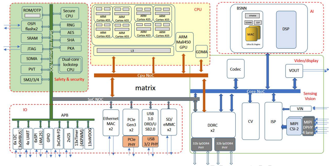
Figure 1-1 Block Diagram
