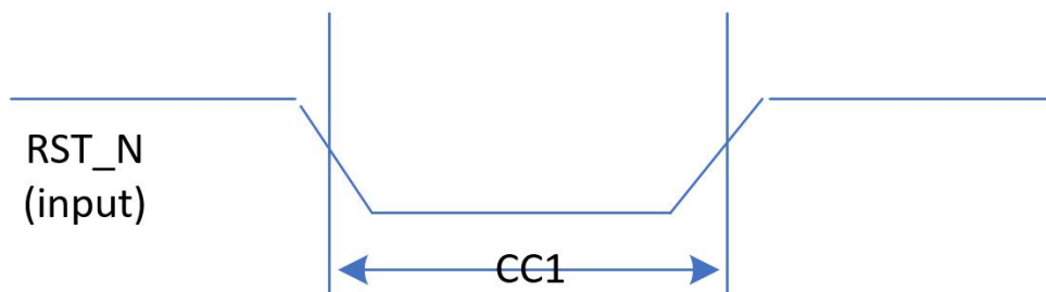
Figure 4-5 Reset timing diagram
