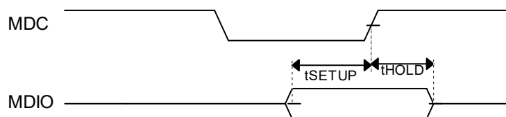
Figure 4-29 MDIO transmit signal timing diagram
