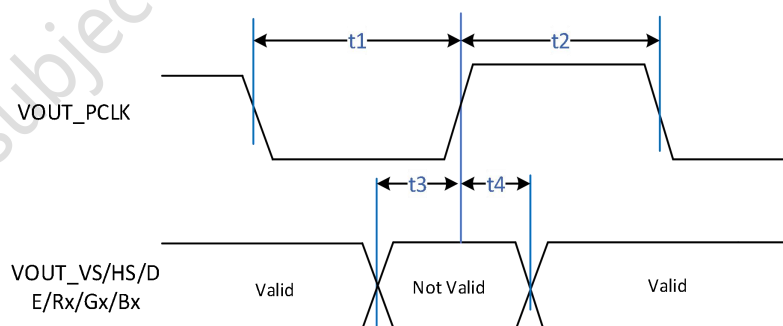
Figure 4-32 VOUT timing diagram
