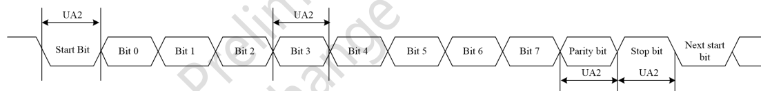
Figure 4-10 UART RS-232 Serial mode receive timing
