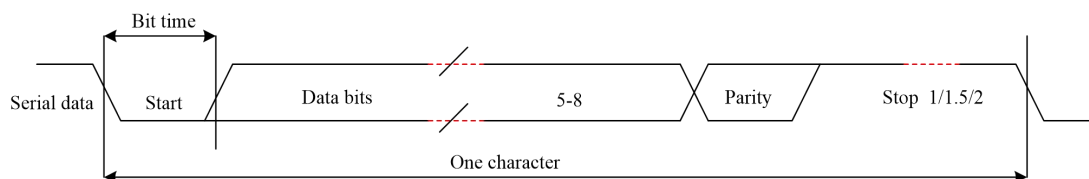
Figure 4-8 Serial data format
