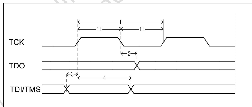
Figure 4-7 JTAG Timing
