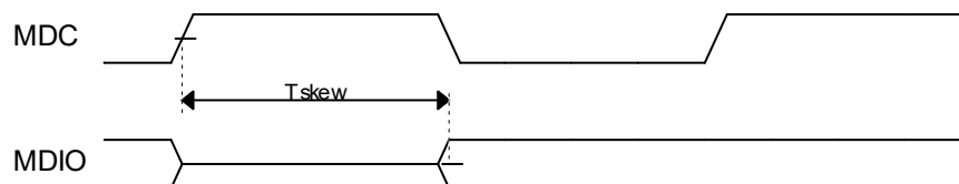
Figure 4-29 MDIO transmit signal timing diagram
