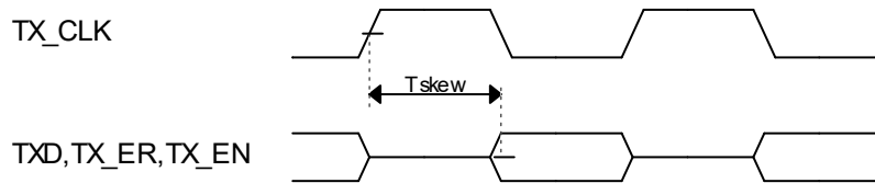
Figure 4-27 MII transmit signal timing diagram
