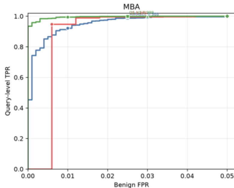
Low-FPR ROC (0-5%): identical benign cohort
