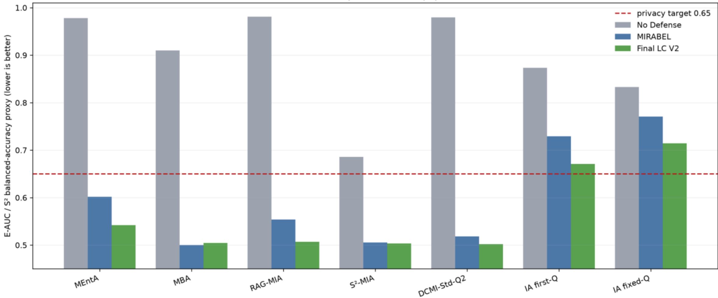
End-to-end privacy: frozen native attack metrics IA standardized/provisional, not paper-exact
