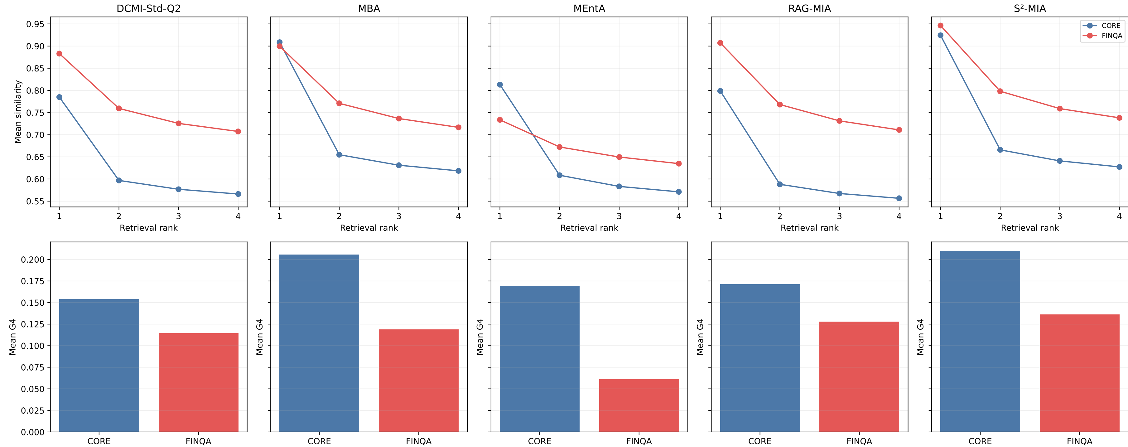
Core vs FinQA frozen retrieval geometry (member queries)
