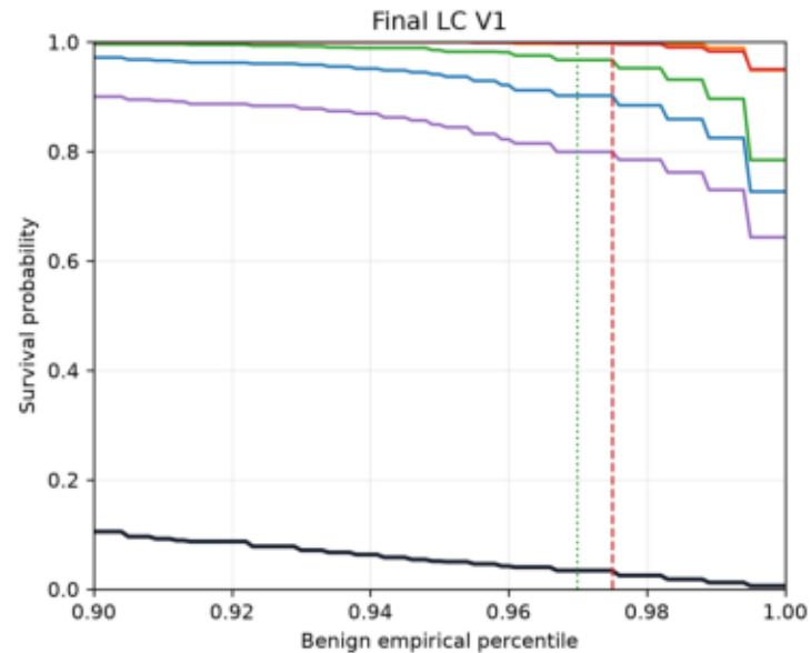
Benign-percentile tail concentration (holdout-CDF diagnostic)
