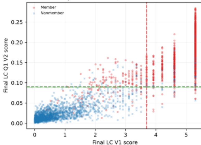
S 2 -MIA Spearman=0.90, Pearson=0.94
