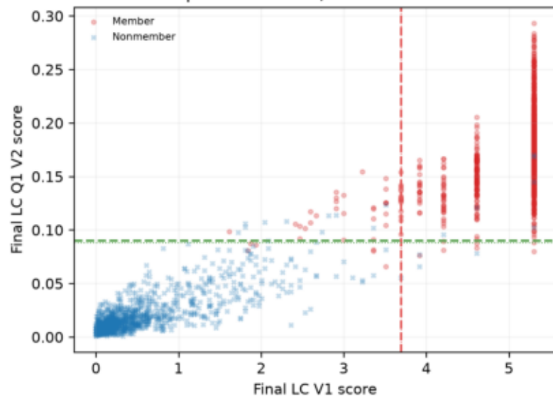
RAG-MIA Spearman=0.91, Pearson=0.95
