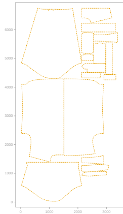
Layer 14 - Sew lines
