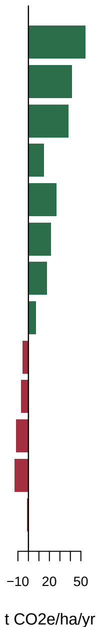
GWP-20
