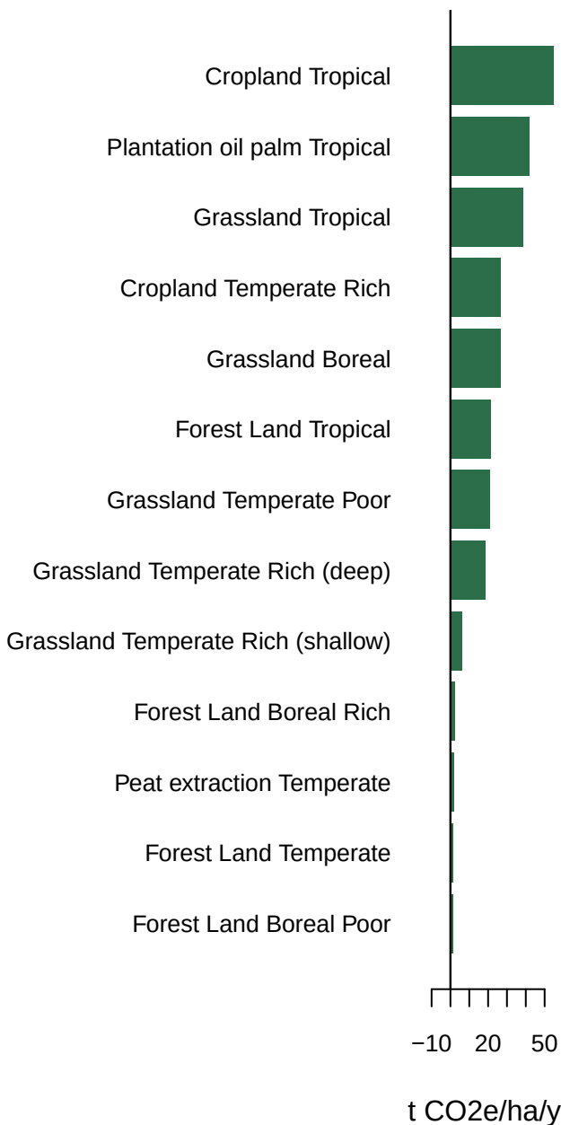
GWP-100
