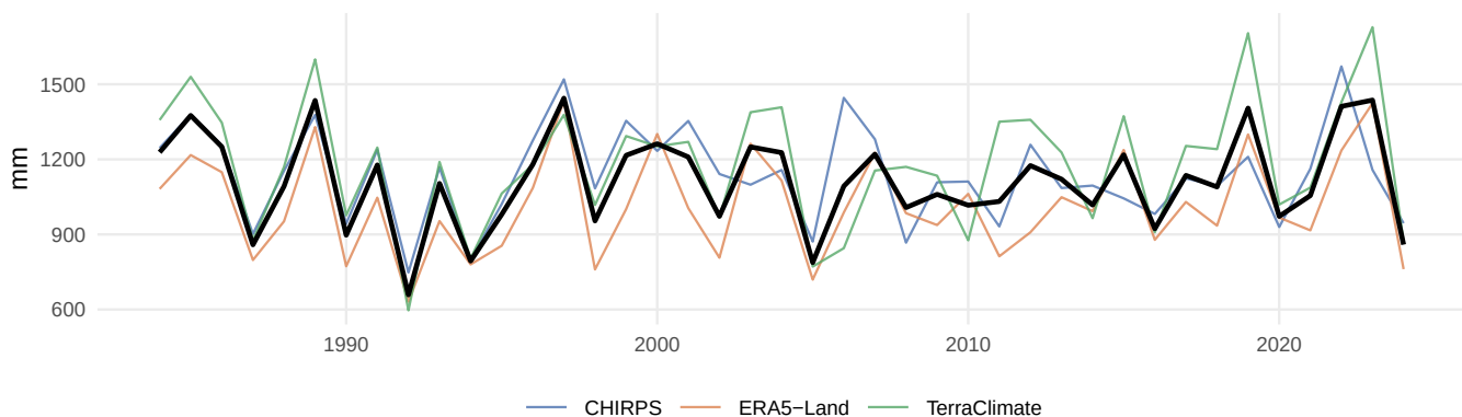
(a) Annual precipitation
