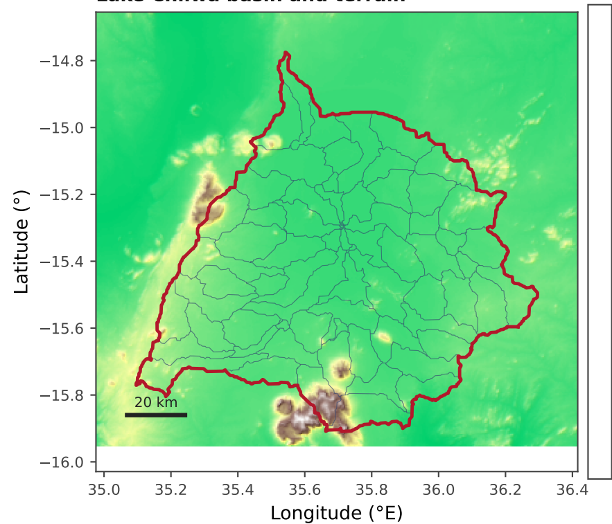
a Lake Chilwa basin and terrain
