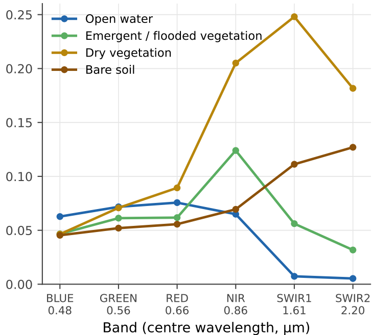
a Image-derived endmember spectra
