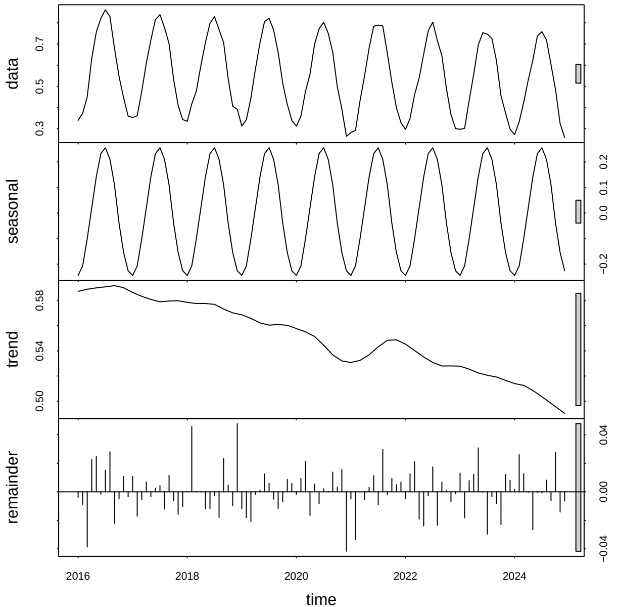
Seasonal-trend decomposition, undisturbed pixel
