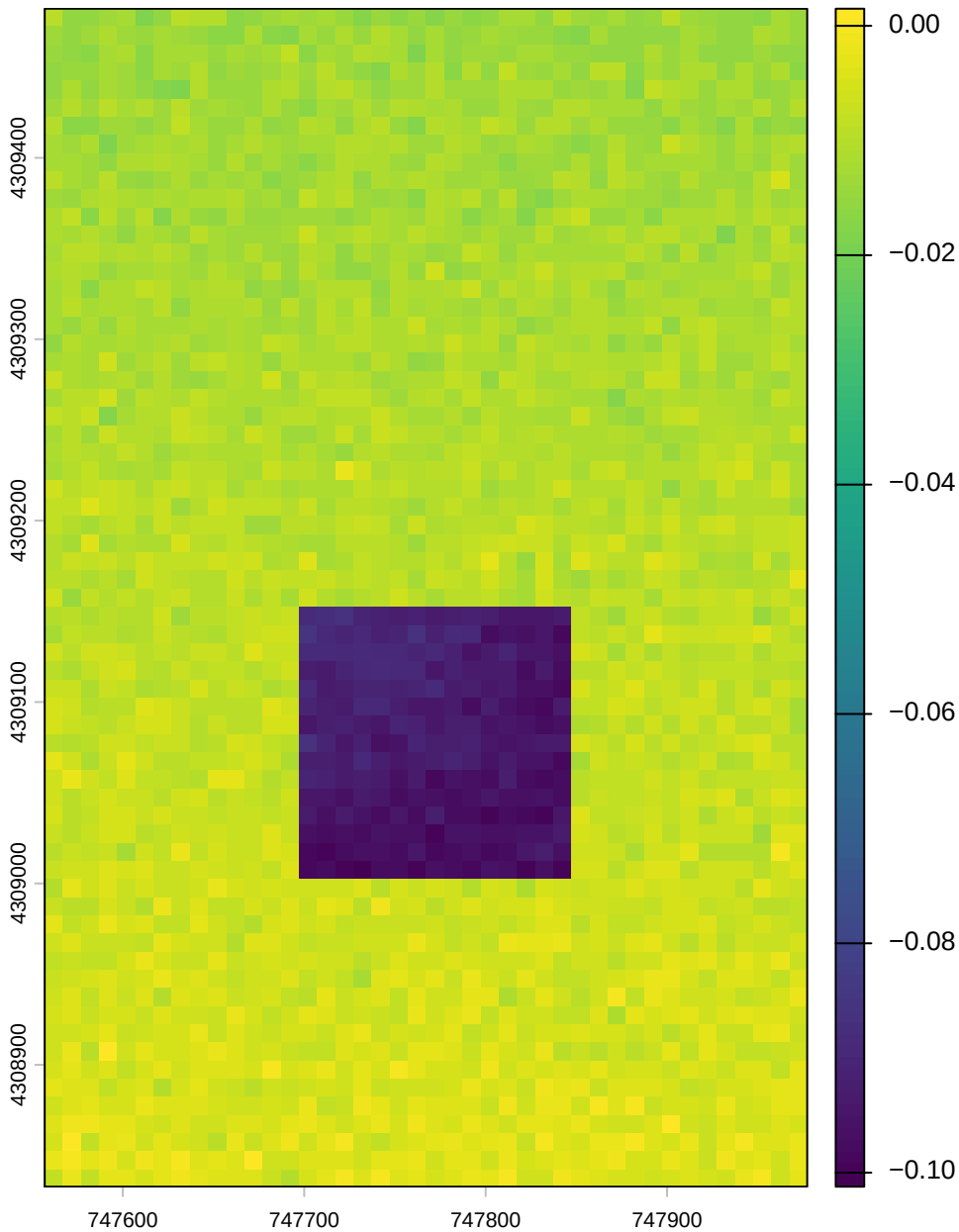
Per-pixel trend (index / year)
