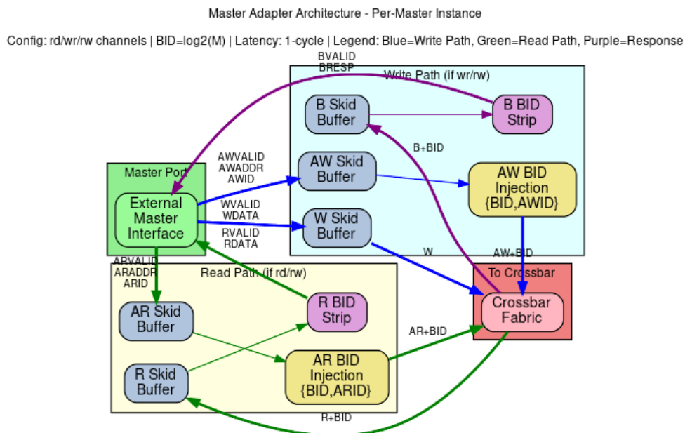
4.2.1 Figure 2.1: Master Adapter Architecture
