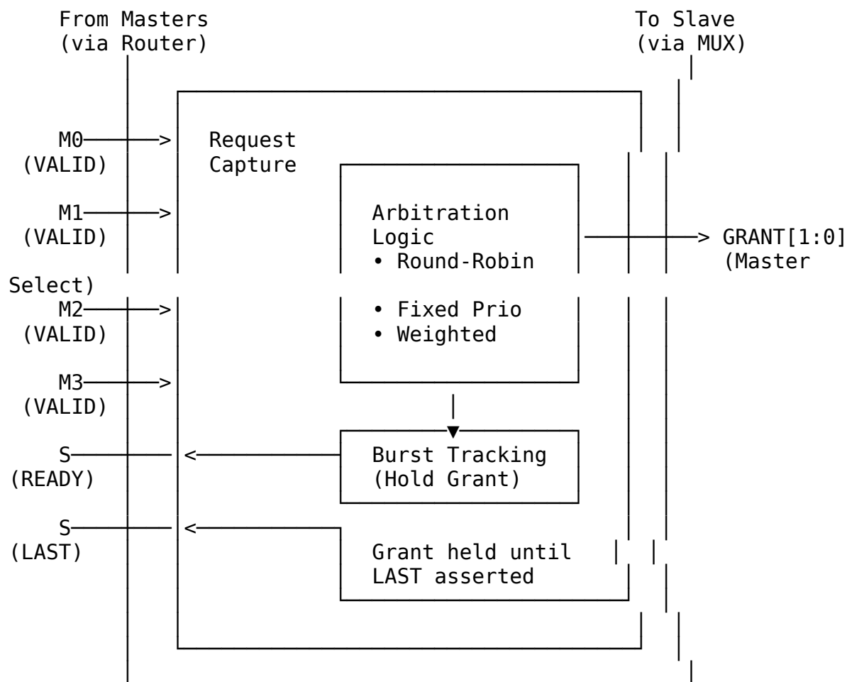
ARBITER (per slave, per channel)
