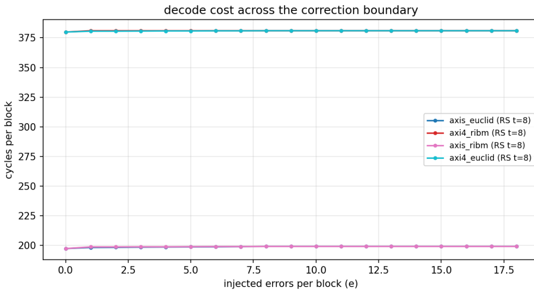
Fig 2: decode cost
